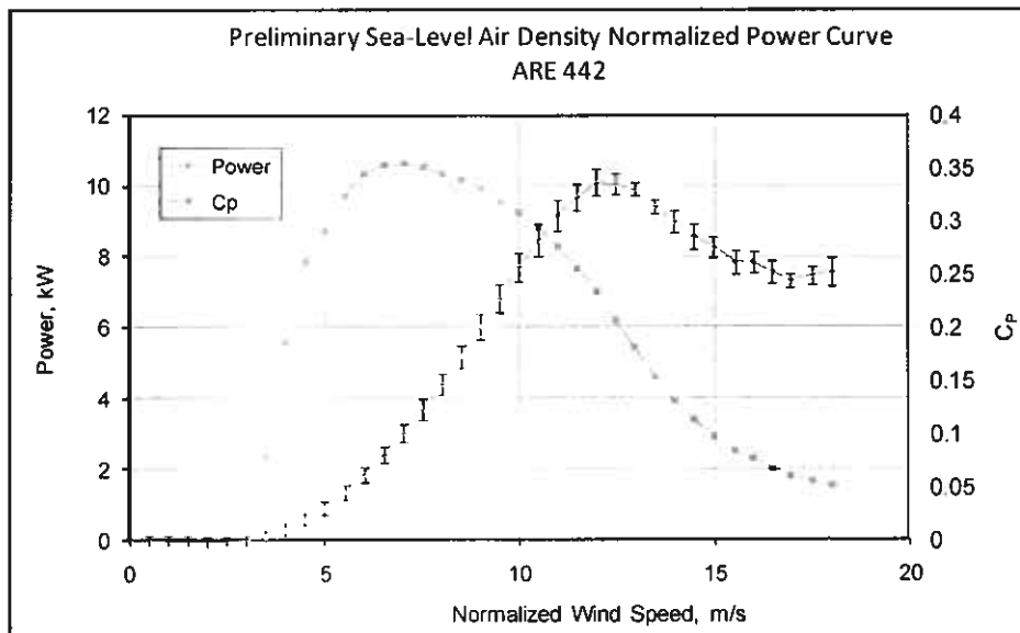
Figure 3. Preliminary power and C_p curves for the ARE 442
