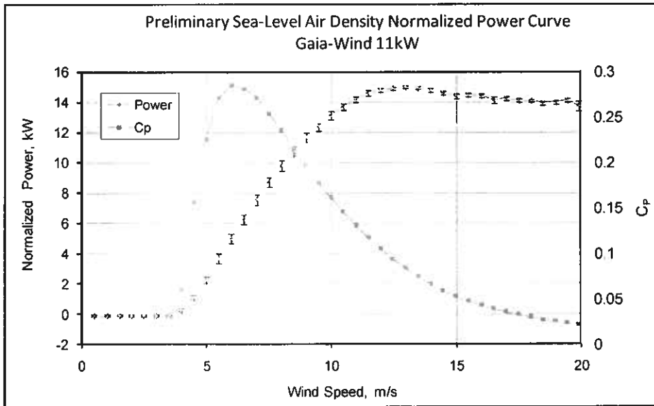
Figure 2. Preliminary power and C_p curves for the Gaia-Wind 11 kW
